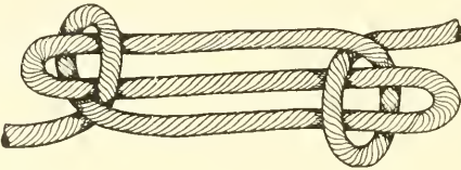
SHEEP SHANK.
